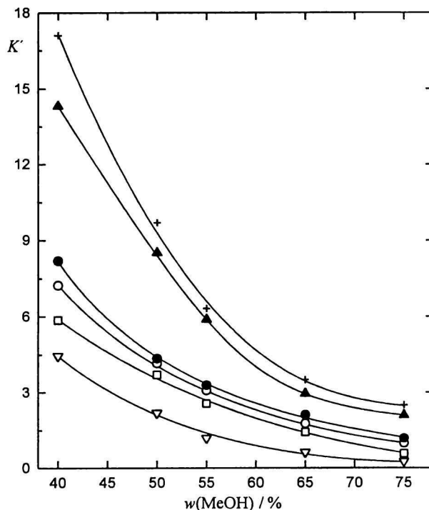
Fig. 1. The influence of methanol content in mobile phase on capacity factors. □ I , ○ II , ▲ III , ▽ AI , ● AII , + AIII .
